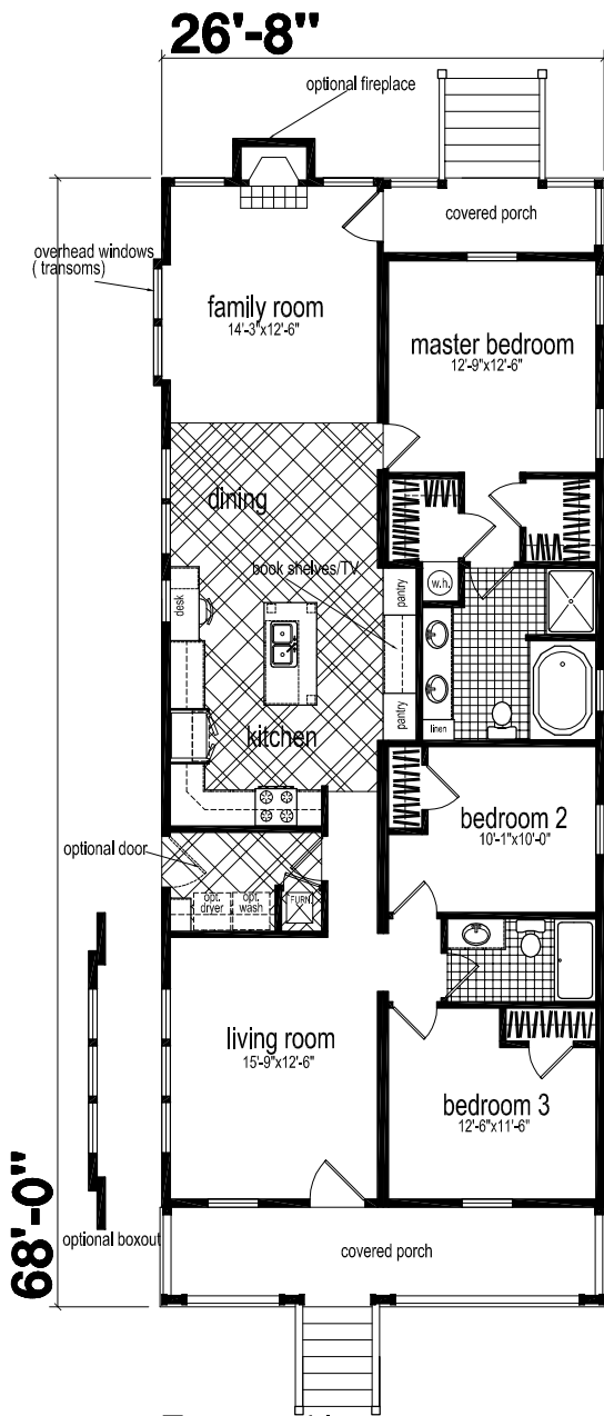
Treywood I model C-418 - 3 bedrooms/2 bathrooms 1833 total sq./ft. (habitable + porches) habitable 1613 sq./ft. covered porches 220 sq./ft.
