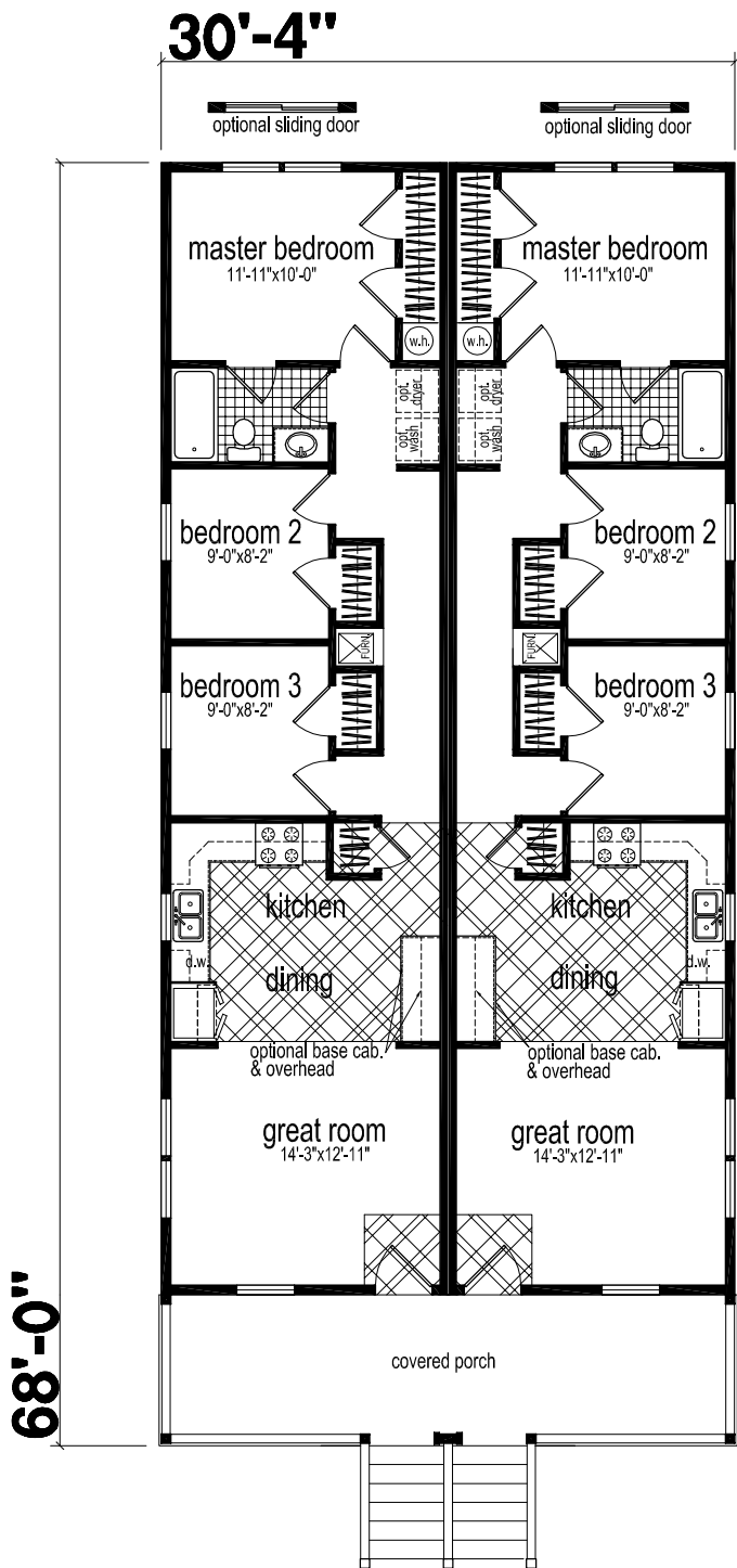
Seabrooke I model C-423 - 3 bedrooms/1 bathroom 2062 total sq./ft. (habitable + porch) habitable 1819 sq./ft. covered porch 243 sq./ft.
